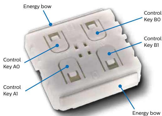
Figure 1 - Outer appearance of PTM 215Z module when the switch cover is removed for switch commissioning.
